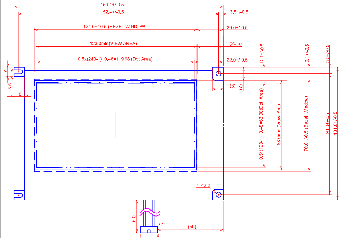
FRONT VIEW
