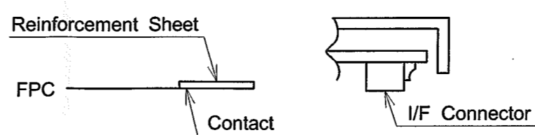
Detail of A-A
