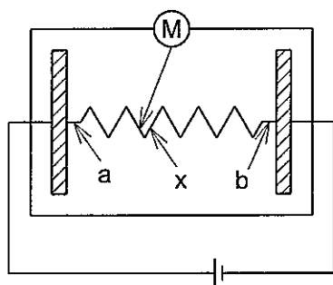
Linearity Definition
