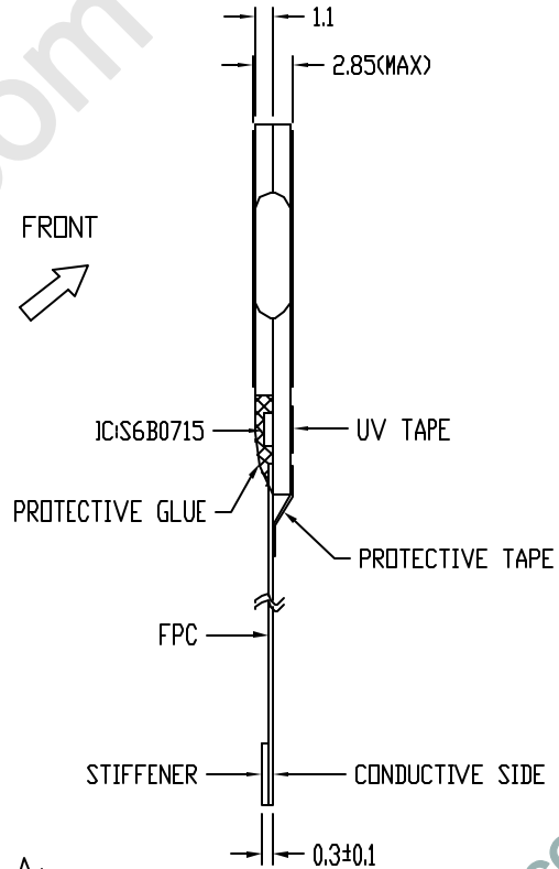
DETAIL B:
