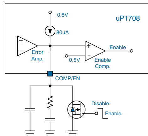
Figure 1. Chip Enable Function
