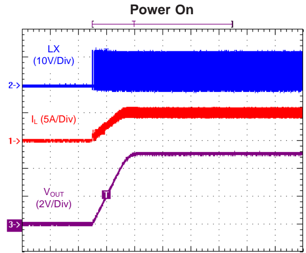
Time (1ms/Div) V IN = 12V, V OUT = 5V, Load = 1Ω
