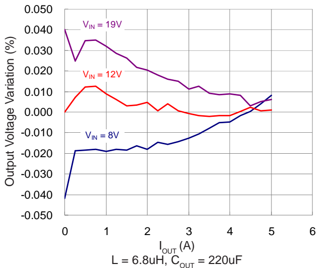
Load Regulation
