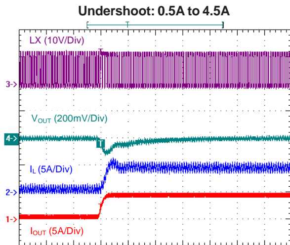
Time (40µs/Div) V IN = 12V, V OUT = 5V, L = 6.8µH, C OUT = 220µF
