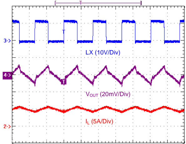
Stability, I_{OUT} = 5A
