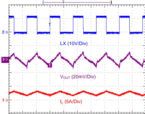
Stability, I_{OUT} = 2.5A
