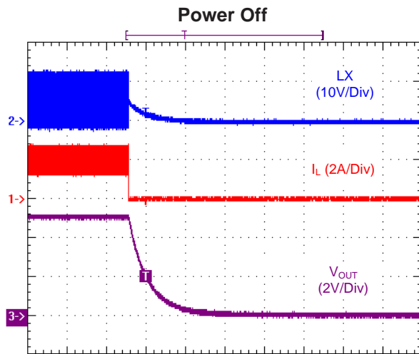
Time (1ms/Div) V IN = 12V, V OUT = 5V, Load = 2.5Ω
