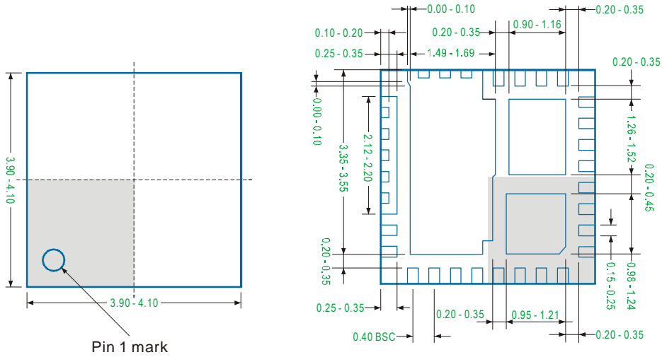
Bottom View - Exposed Pad
