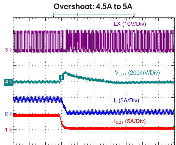
Time (40µs/Div) V IN = 12V, V OUT = 5V, L = 6.8µH, C OUT = 220µF
