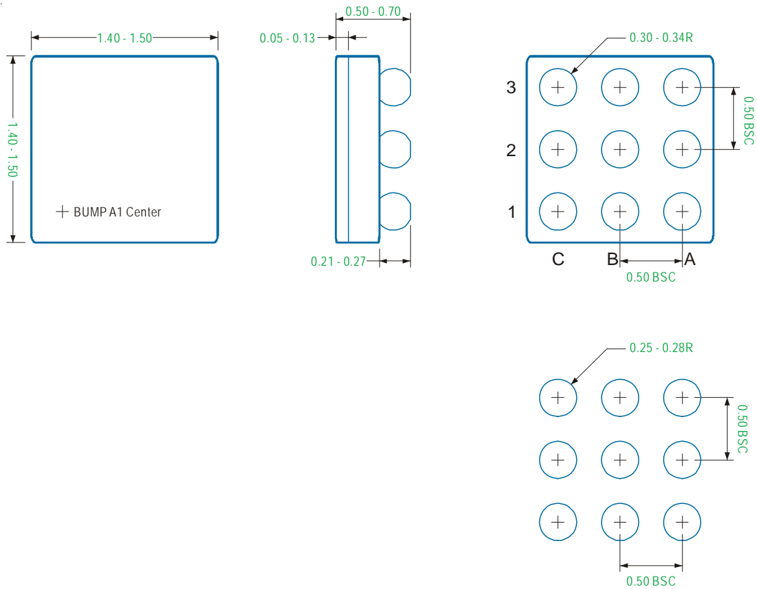
Recommended Solder Pad Layout
