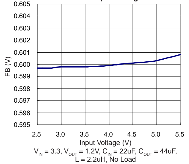
Line Regulation vs. Input Voltage
