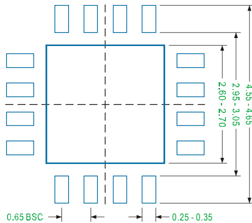
Recommended Solder Pad Pitch and Dimensions
