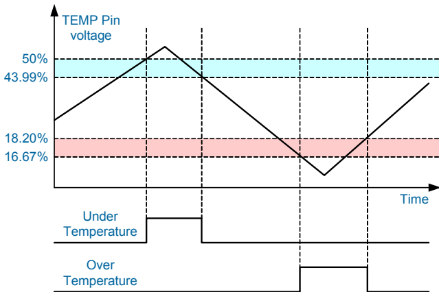
Figure 3. Battery Temperature Monitoring.
