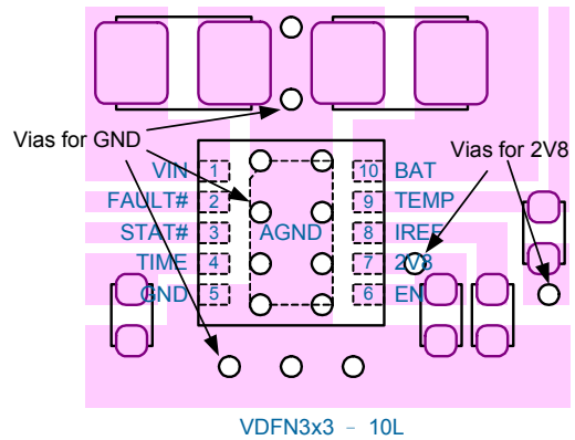
Figure 1. Top Layer Layout Examples
