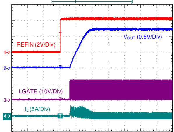
Time : 2ms/Div V_{IN} = 12V, V_{OUT} = 1.2V, C_{OUT} = 2000\mu F, \text{No Load}
