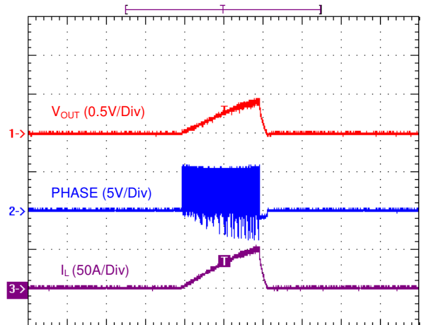
Time : 400us/Div V_{IN} = 12V , V_{OUT} = 1.2V , C_{OUT} = 2000\mu F , Short V_{OUT} \Rightarrow Power On
