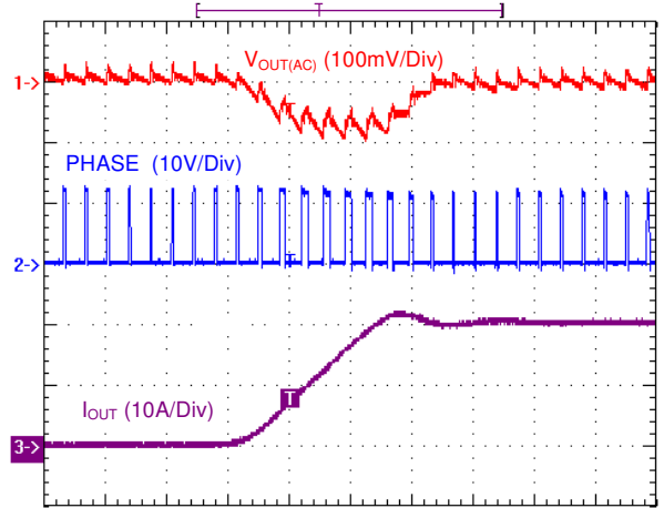
Time : 10us/Div V_{IN}=12V , V_{OUT} = 1.2V , C_{OUT} = 2000\mu F
