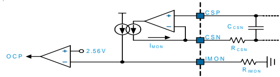
Figure 7. Total Output OCP
