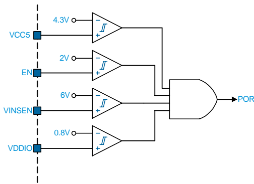
Figure 1. Circuit for Power Ready Detection
