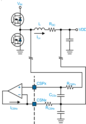
Figure 8. Phase Current Sense
