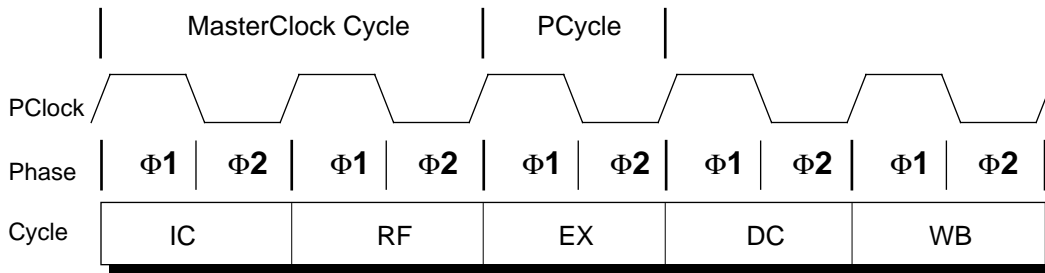
Figure 4-1 Pipeline Stages
