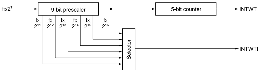
Figure 5-6. Block Diagram of Watch Timer
