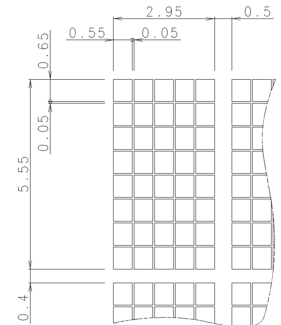
DOT DETAIL SCALE 10:1
