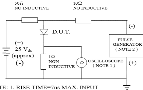
FIG. 1-TEST CIRCUIT DIAGRAM AND REVERSE RECOVERY TIME CHARACTERISTIC
