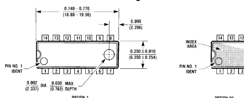
Cavity Dual-In Line Package (J) Order Number MM54HC00J or MM74HC00J NS Package J14A
