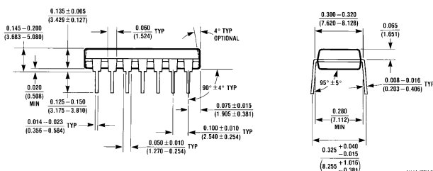
Molded Dual-In Line Package (N) Order Number MM74HC00N NS Package N14A
