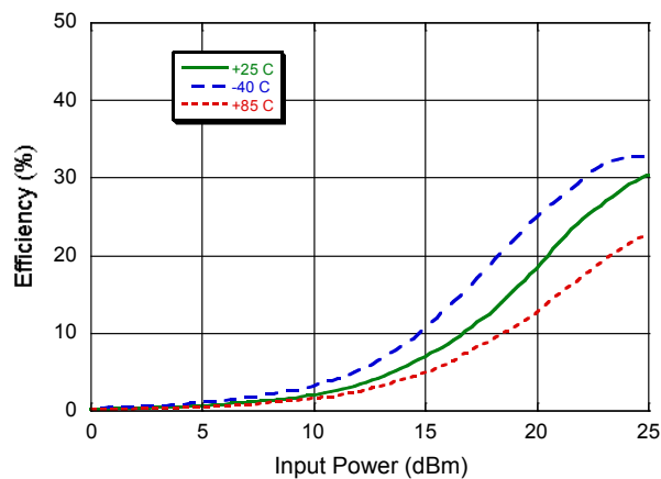
Efficiency @ 4 GHz
