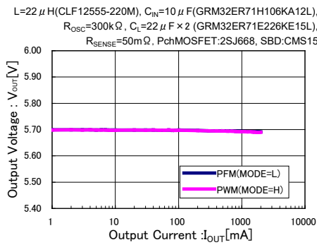
XC9252x08A ( V_{IN}=12V , V_{OUT}=5.7V , f_{OSC}=280kHz )
