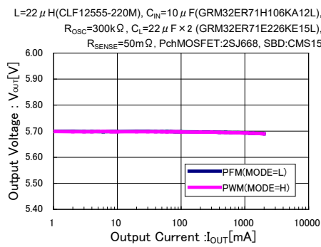
XC9252x08A ( V_{IN}=24V , V_{OUT}=5.7V , f_{OSC}=280kHz )
