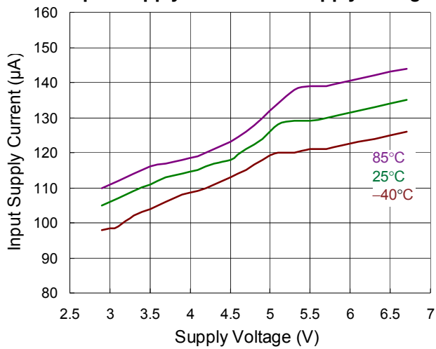
Input Supply Current vs. Supply Voltage
