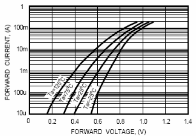
FIG. 2 - FORWARD CHARACTERISTICS
