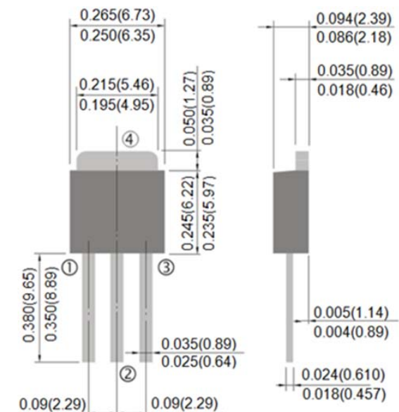
TO-251AA Dimension
