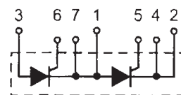
MCC44I01B
