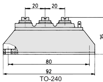
TO-240
