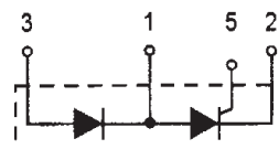
MCD26I08B
