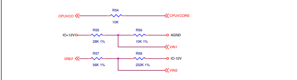
Voltage Sensing
