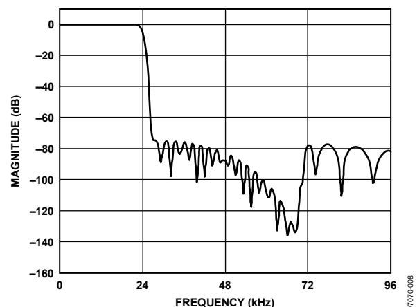
Figure 11. DAC Pass-Band Filter Response (48 kHz)
