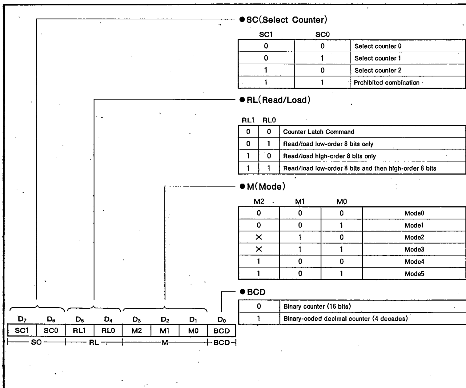
Fig. 1 Control-Word Format
