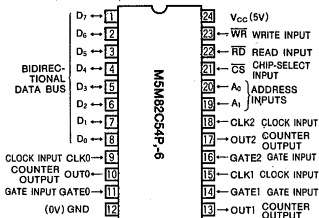
Outline 24P4
