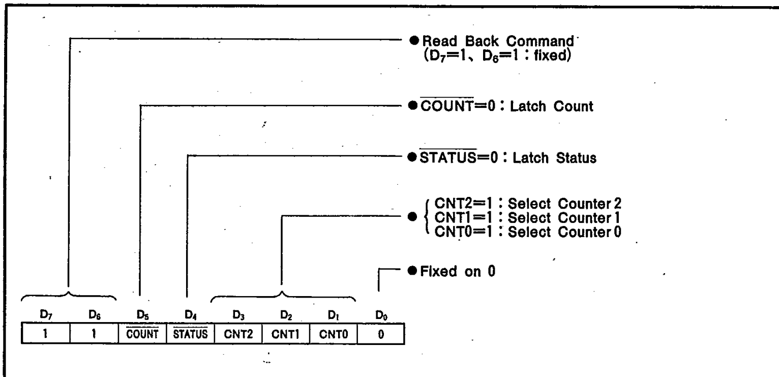
Fig. 8 Read Back Command Format
