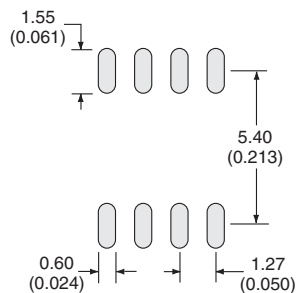
Recommended PCB Land Pattern
