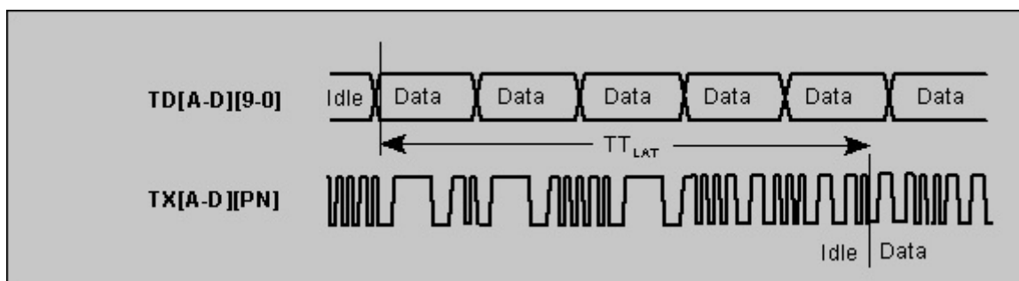
FIGURE 6-2. TRANSMITTER LATENCY
