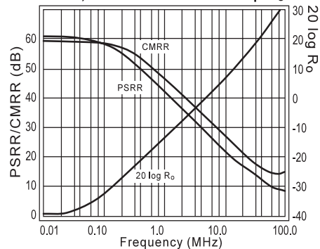
PSRR, CMRR and Closed Loop R_o
