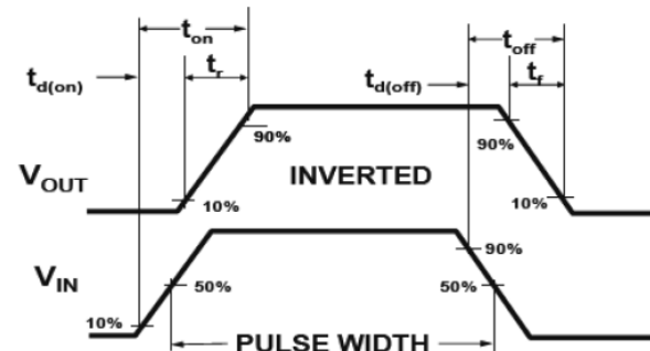
Switch Waveforms:
