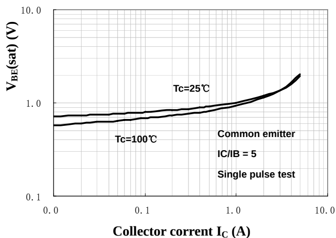
Base-Emitter Voltage
