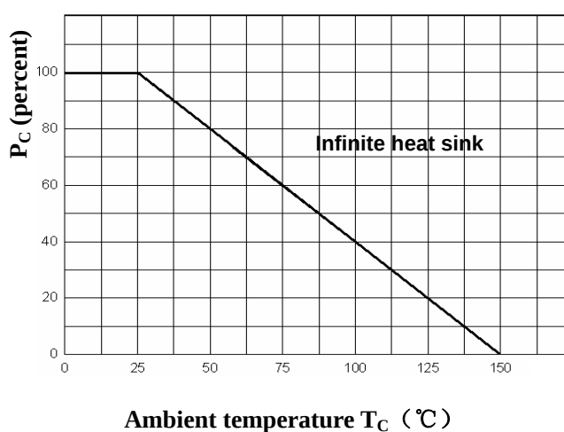
Power Derating
