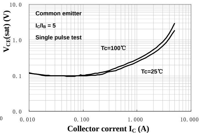
Saturation Voltage
