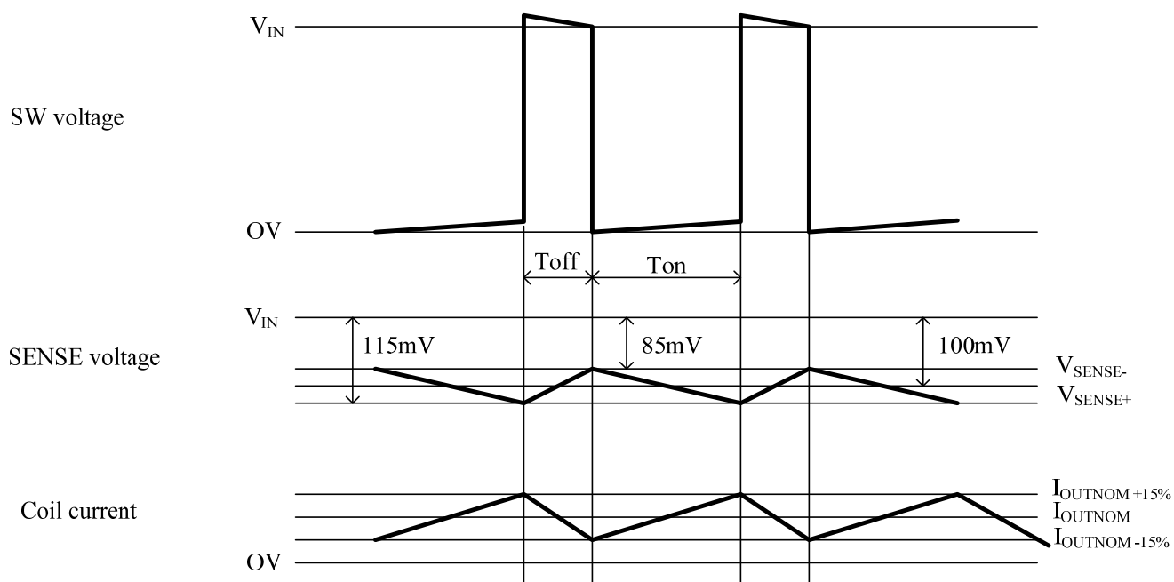
Figure 1-Operating waveforms
