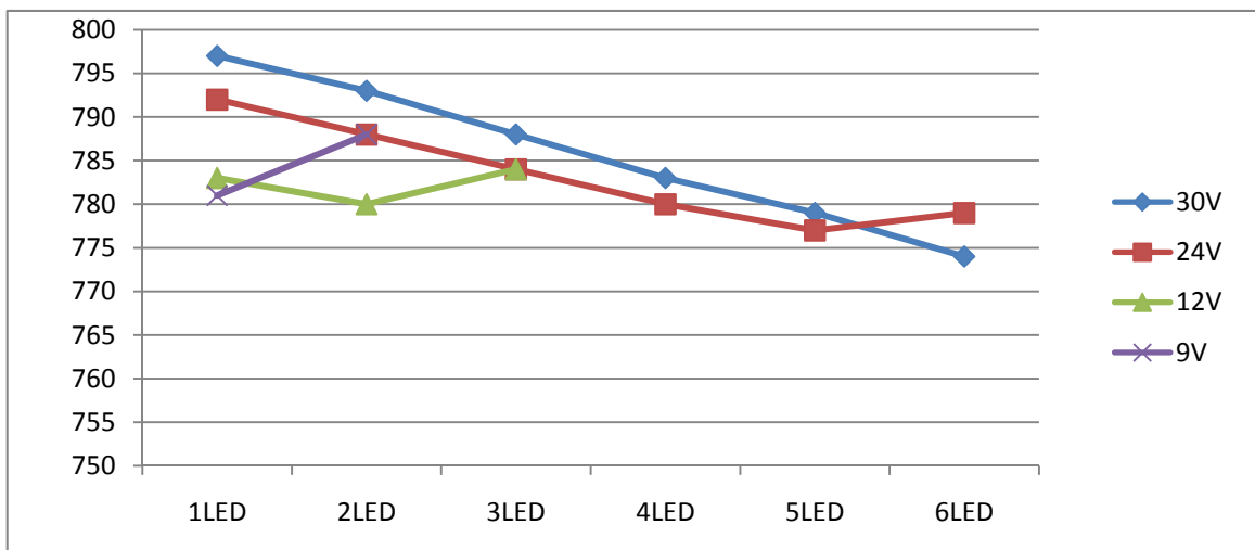
Output current vs. LED cascaded number @L=68uH、I OUT =770mA
