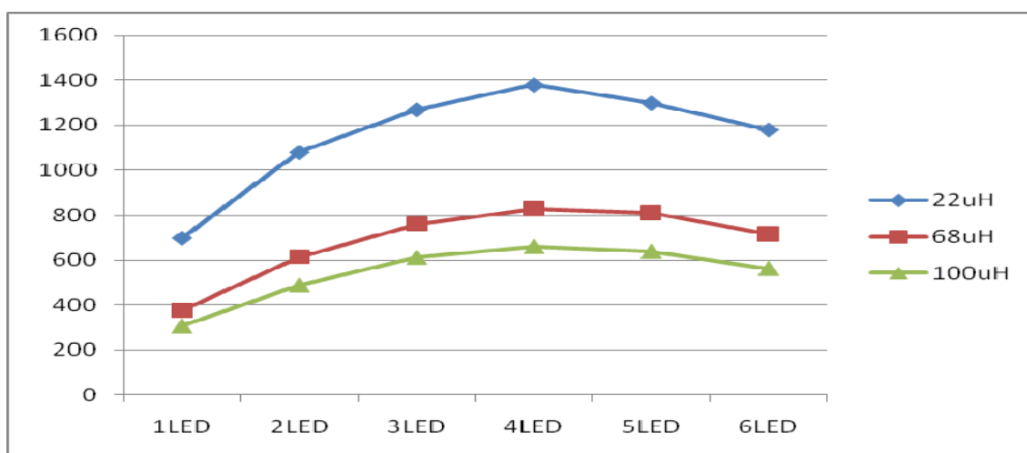
Switching Frequency vs. LED Cascaded Number @VIN=30V、I OUT =370mA
