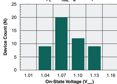
Typical On-State Voltage Distribution ( I_L=1\text{A}_{\text{rms}} , T_A=25^\circ\text{C} )
