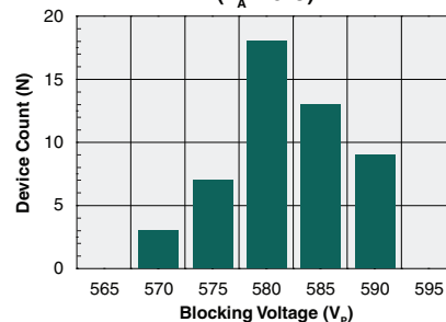
Typical Blocking Voltage Distribution ( T_A=25^\circ\text{C} )
