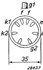
Fig. 2 Arrangement of electrodes and base connections.
