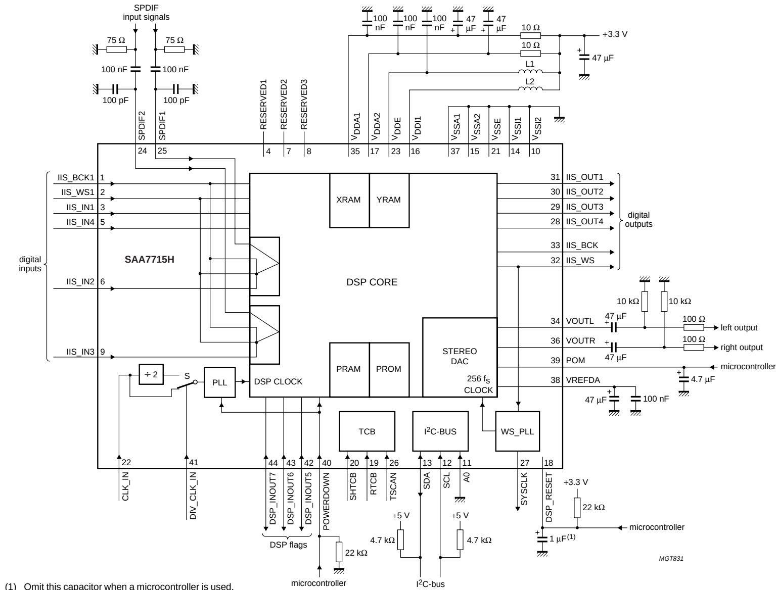
Fig.11 Application diagram.
