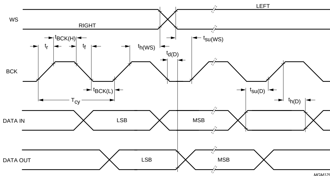
Fig.9 Timing of the digital audio data inputs and outputs.
