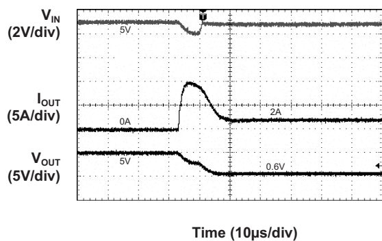
Short Circuit Through 0.3 \Omega Response
