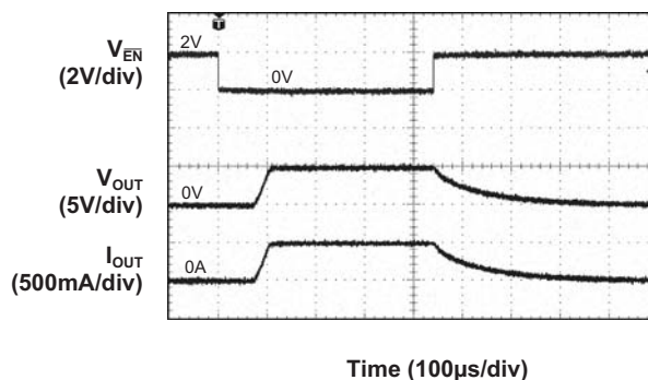
Turn-On/Off Response ( R_{OUT} = 10\Omega ; V_{MAIN} = 5V )
