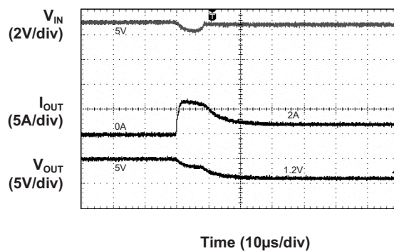
Short Circuit Through 0.6 \Omega Response
