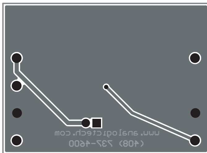
Figure 3: AAT4672 Evaluation Board Bottom Side Layout.
