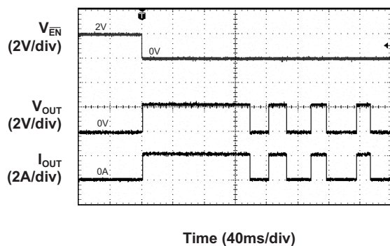
Thermal Shutdown Response ( V_{\text{MAIN}} = 5\text{V} )
