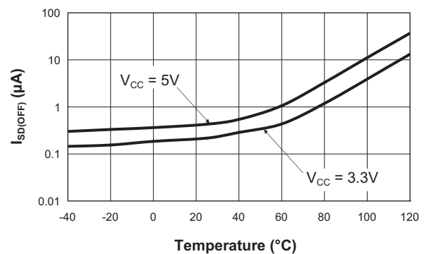
Off-Switch Current vs. Temperature ( ENIU = ENIL = \text{High} ; V_{OUT} = 0V )
