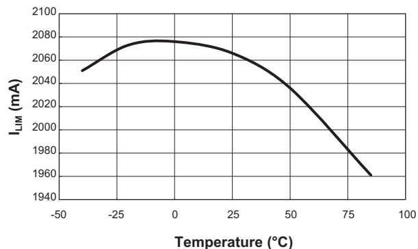
AAT4621-1 I_{LIM} vs. Temperature ( V_{CC} = 5V ; V_{OUT} = 4.5V ; ENIU = 0V ; R_{SETU} = 1.24M\Omega )
