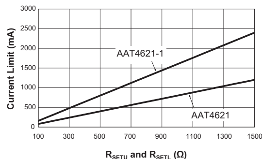
Figure 1: Calculated Current Limit R_{SET} Characteristic.
