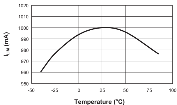
AAT4621 I_{LIM} vs. Temperature ( V_{CC} = 4V ; V_{OUT} = 3.85V ; ENIU = 0V ; R_{SETU} = 1.3M\Omega )
