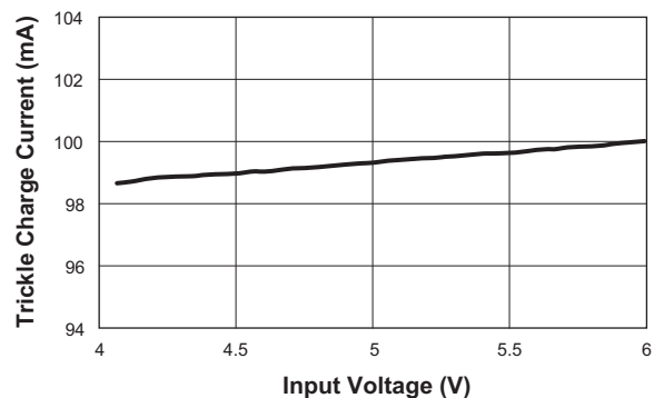
Trickle Charge Current vs. Input Voltage ( R_{\text{SENSE}} = 0.2\Omega ; 1.8X Mode)
