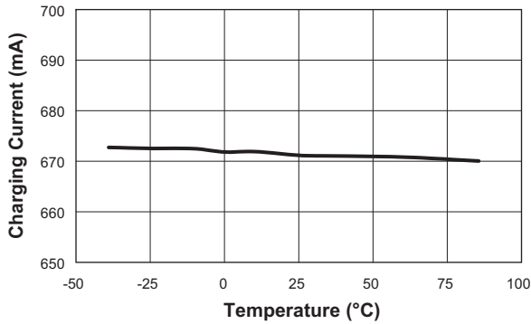
Charging Current vs. Temperature ( R_{\text{SENSE}} = 0.15\Omega )
