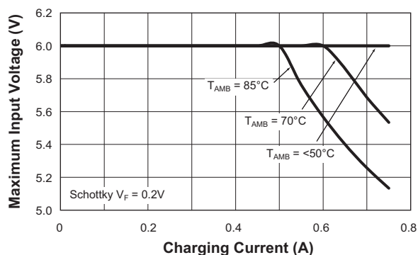
Safe Operating Area ( T_{\text{J(MAX)}} = 150^\circ\text{C} )
