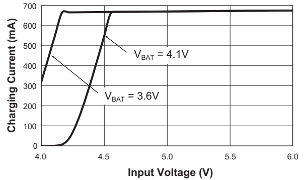
Charging Current vs. Input Voltage ( R_{\text{SENSE}} = 0.15\Omega with External Schottky)
