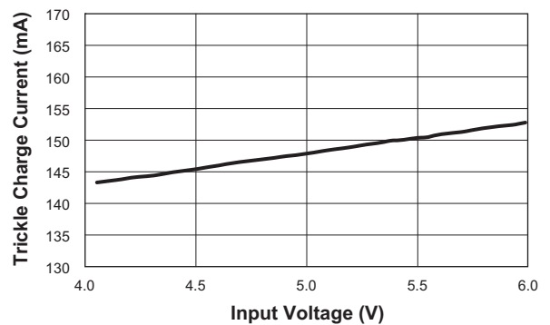
Trickle Charge Current vs. Input Voltage ( R_{\text{SENSE}} = 0.15\Omega ; 1.8X Mode)
