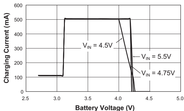
Charging Current vs. Battery Voltage ( R_{\text{SENSE}} = 0.2\Omega with External Schottky)
