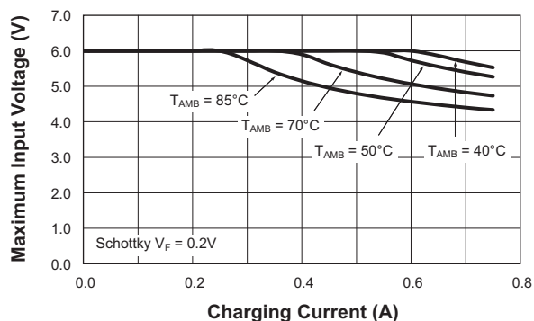
Safe Operating Area ( T_{\text{J(MAX)}} = 120^\circ\text{C} )
