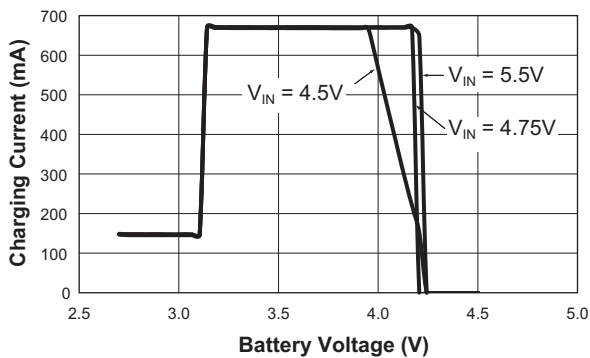
Charging Current vs. Battery Voltage ( R_{\text{SENSE}} = 0.15\Omega with External Schottky)
