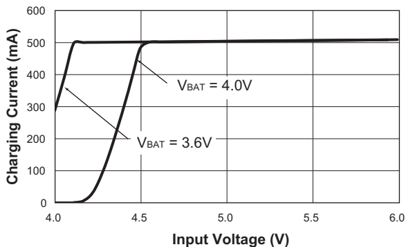
Charging Current vs. Input Voltage ( R_{\text{SENSE}} = 0.2\Omega with External Schottky)
