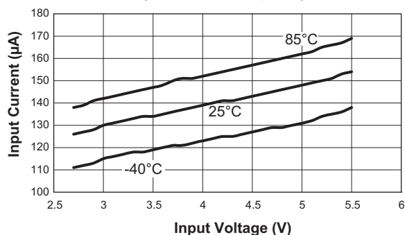
Step-Down Converter and LDO Input Current vs. Input Voltage
