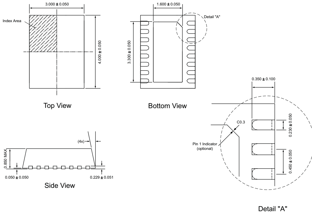
TDFN34-16 3
