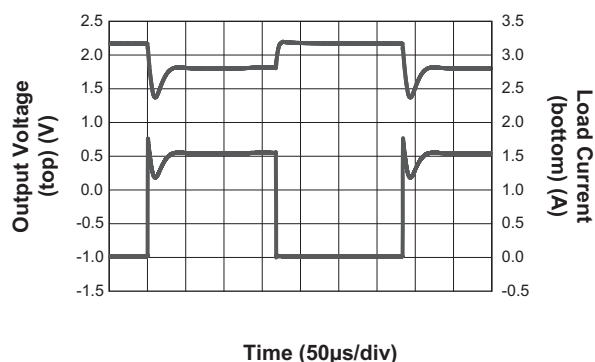
Load Transient Response ( V_{IN} = 3.6V ; V_{OUT} = 1.8V ; No C_{FF} )
