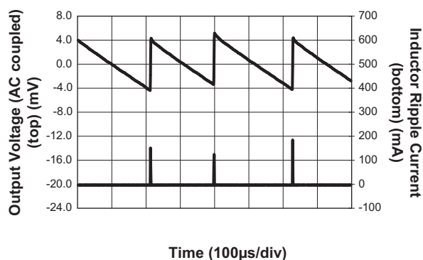
Light Load Switching Waveform (Light-Load Mode; V_{IN} = 3.6V ; V_{OUT} = 1.8V ; 1mA Load)
