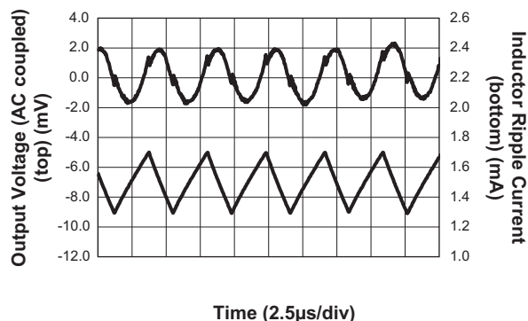
Heavy Load Switching Waveform (PWM Mode; V_{IN} = 3.6V ; V_{OUT} = 1.8V ; 1.5A Load)
