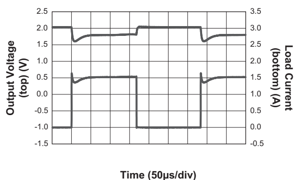
Load Transient Response ( V_{IN} = 3.6V ; V_{OUT} = 1.8V ; C_{FF} = 100pF )
