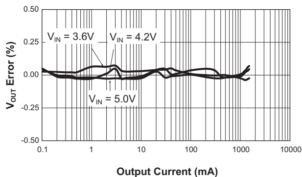
Load Regulation (Light-Load Mode; V_{OUT} = 3.3V )
