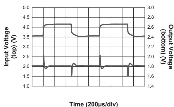
Line Transient Response ( V_{OUT} = 1.8V ; 1.5A Load)
