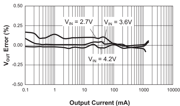
Load Regulation (Light-Load Mode; V_{OUT} = 2.5V )
