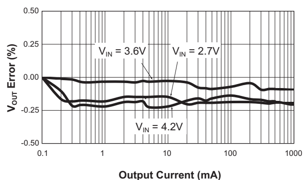
Load Regulation (Light-Load Mode; V_{OUT} = 1.8V )
