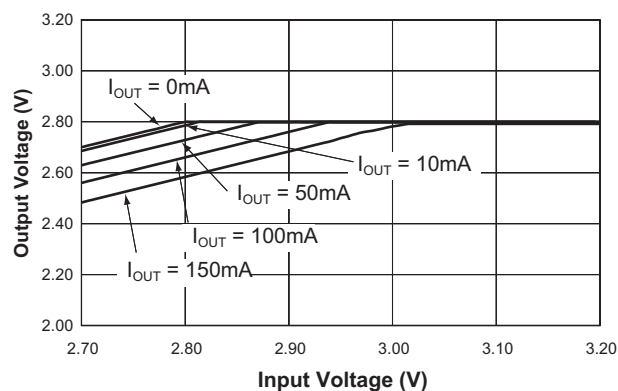
Dropout Characteristics
