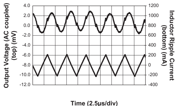
Light Load Switching Waveform (PWM Mode; V_{IN} = 3.6V ; V_{OUT} = 1.8V ; 1mA Load)
