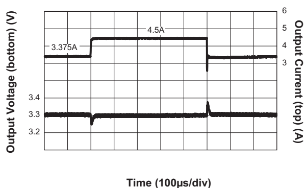
Step-Down Converter Load Transient Response ( I_{OUT1} = 3.375A to 4.5A ; V_{IN1} = 12V ; C_{OUT1} = 3x22μF )
