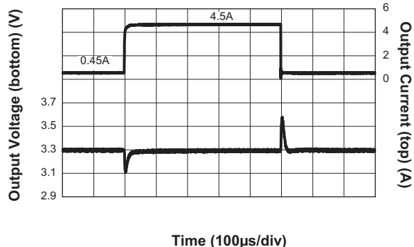
Step-Down Converter Load Transient Response ( I_{OUT1} = 0.45A to 4.5A ; V_{IN1} = 12V ; C_{OUT1} = 3x22μF )
