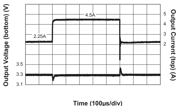
Step-Down Converter Load Transient Response ( I_{OUT1} = 2.25A to 4.5A ; V_{IN1} = 12V ; C_{OUT1} = 3x22μF )
