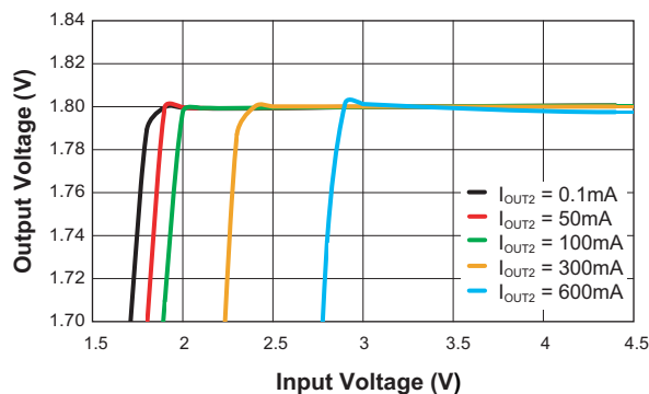
LDO Dropout Characteristics
