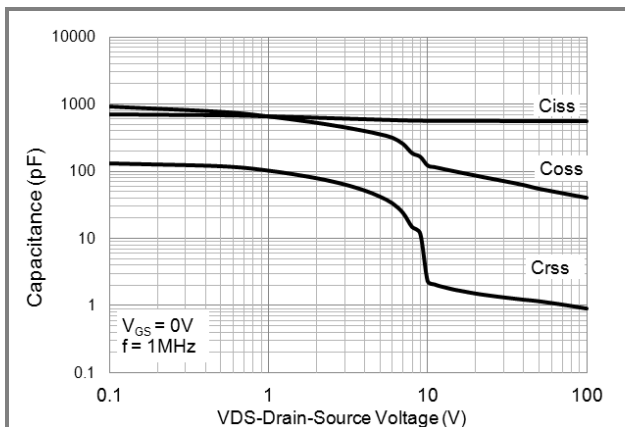
Fig.5 Capacitance vs. Drain-Source Voltage
