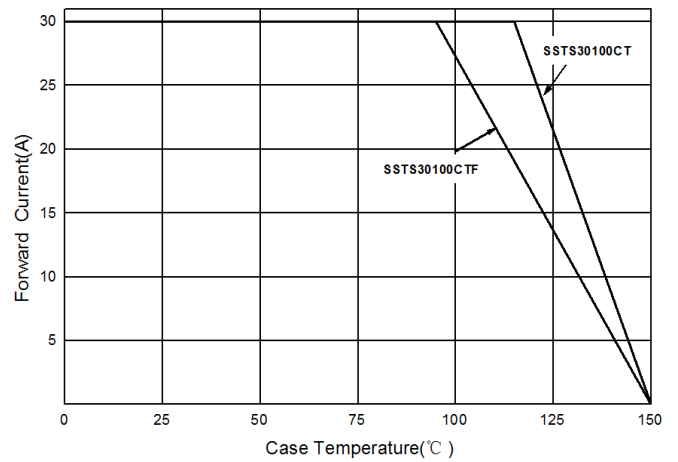
Figure 4: Forward Current Derating Curve
