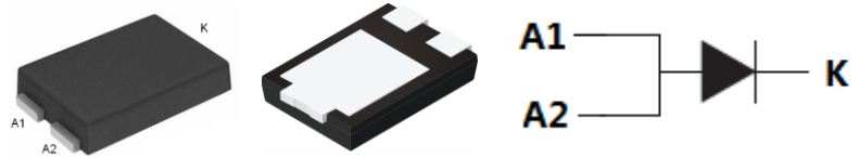
TO-277
