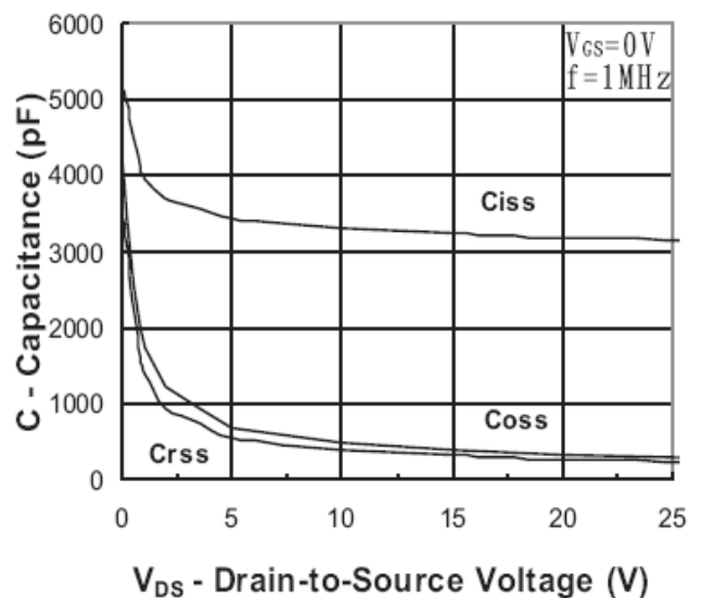
Capacitance
