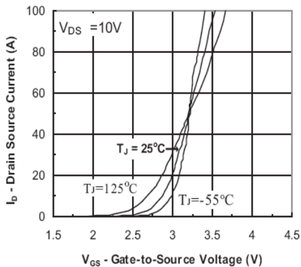
Transfer Characteristic
