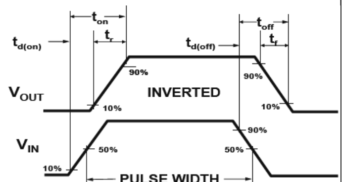
Switch Waveforms:
