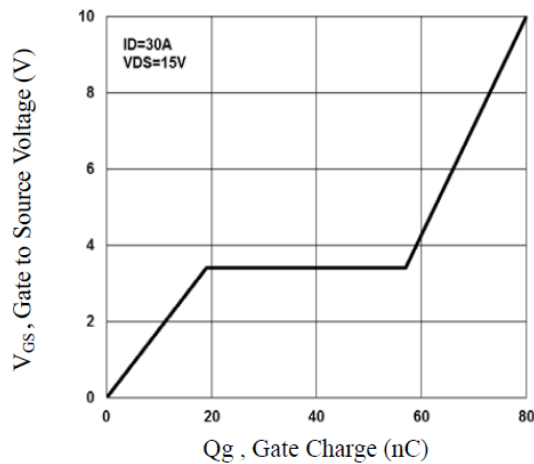
Figure 3: Gate-Charge Characteristics
