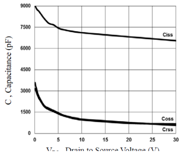
Figure 4: Capacitance Characteristics
