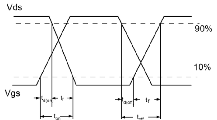
Waveforms:
