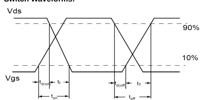
Switch Waveforms:
