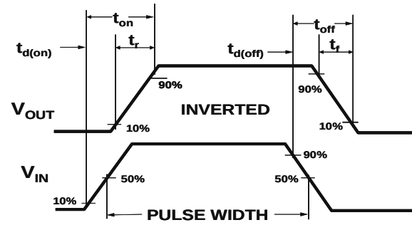
Figure 2: Switching Waveforms
