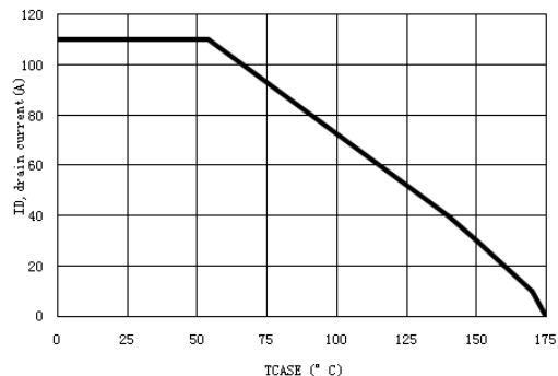
Figure 12: Current De-rating (3)
