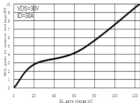
Figure 7: Gate-Charge Characteristics Figure
