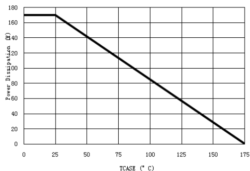
Figure 11: Power De-rating (3)
