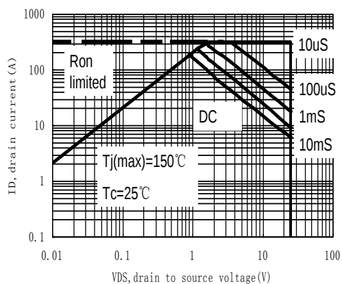
Figure 9: Maximum Forward Biased Safe Operating Area(5)
