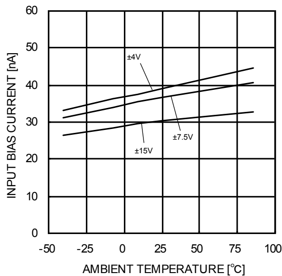
Figure 13. Input Bias Current - Ambient Temperature ( V_{ICM}=0V, V_{OUT}=0V )
