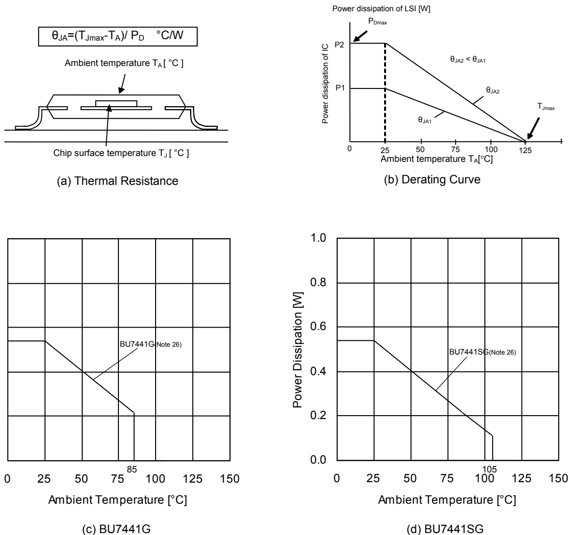
Figure 78. Thermal Resistance and Derating Curve
