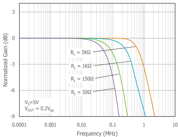
Freq. Resp. vs. R_L +5V
