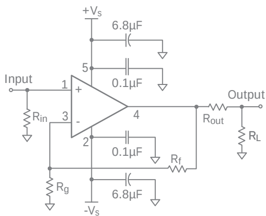
Figure 7. CEB004 Schematic
